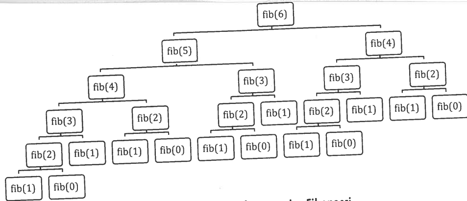
Figure 13.1 Tree of calls for recursive Fibonacci
